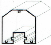
SPB100 Sign Post Bevel-100 mm Stock Length: 6010 mm (UK) 8' or 12' (US) (APG200E)
