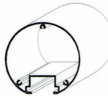
SPC100 Sign Post Circular-100 Stock Length: 6010 mm (UK) 8' or 12' (US) (APG138)
