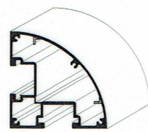
SPQ100 Sign Post Quarter Round - 100mm Stock Length: 6010 mm (UK) 8' or 12' (US) (APG163)
